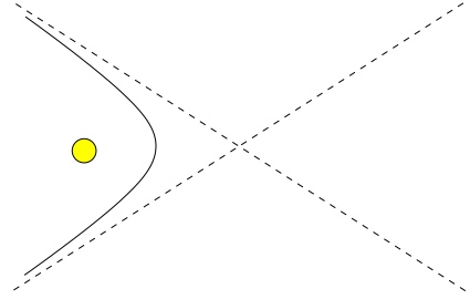
Figure 17: A hyperbola
