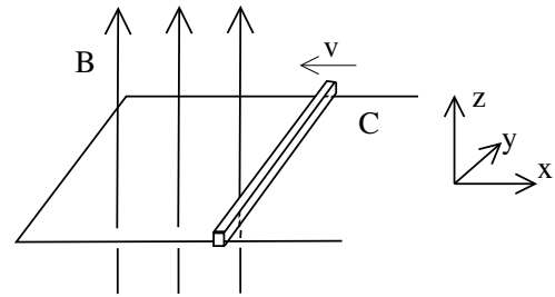
Figure 36: Moving circuit
