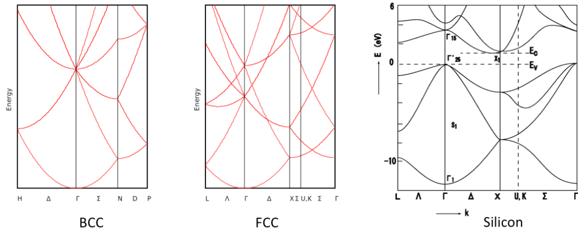
Figure 32: Free band structure (in red) for BCC and FCC, together with the band structure for silicon, exhibiting a gap.
